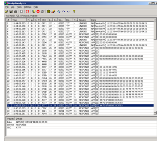
Figure 1: GadgetAnalyzer Packet Log
