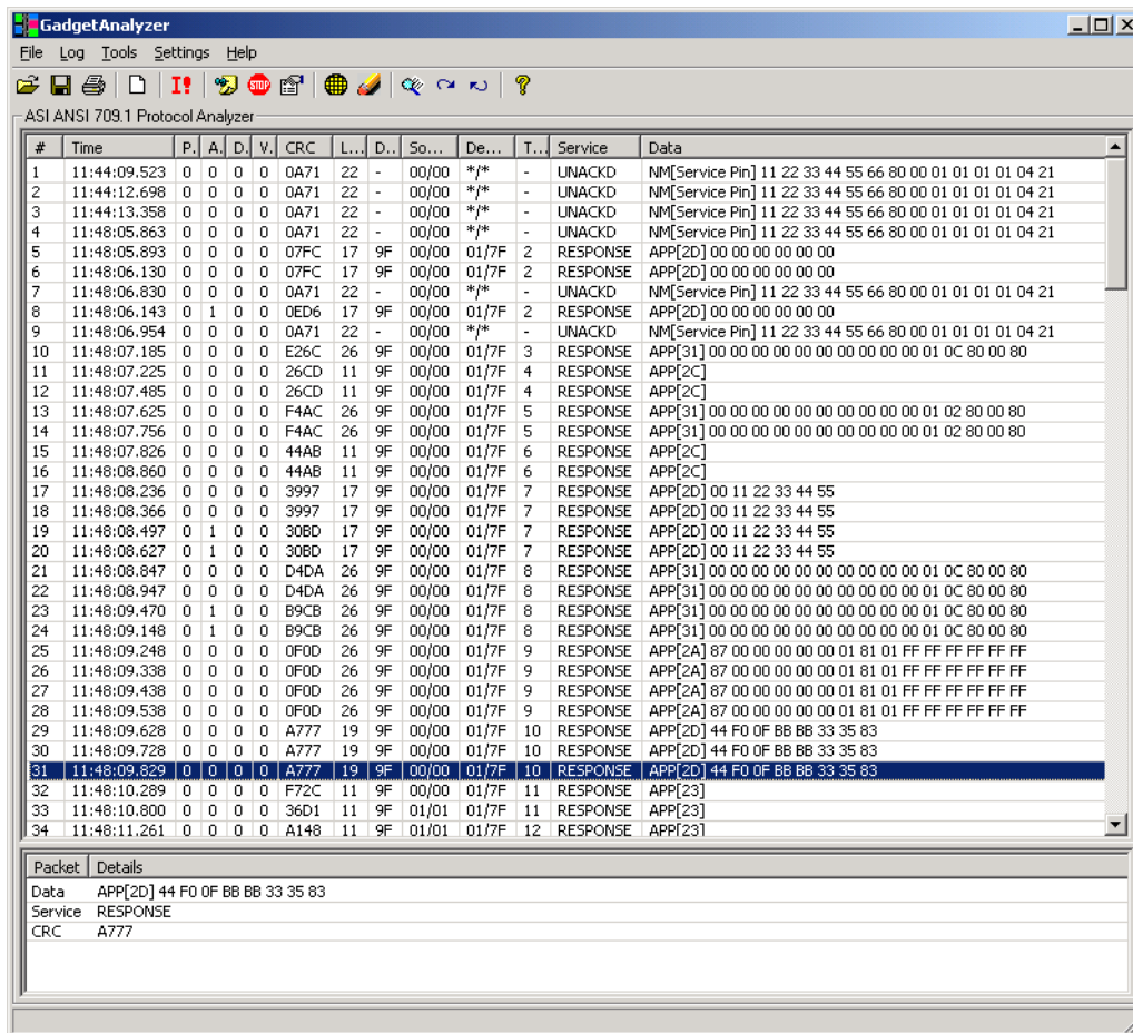
Figure 2: Packet Log Screen Display for GadgetAnalyzer
